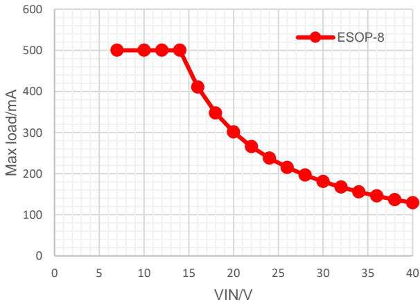
Figure 28. Maximum Output Current vs Input Voltage, VOUT=5V of ESOP-8, T_J \leq TSD\_R(4\text{-layer EVM})
